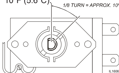
Fig. 11 Adjust Thermostat
