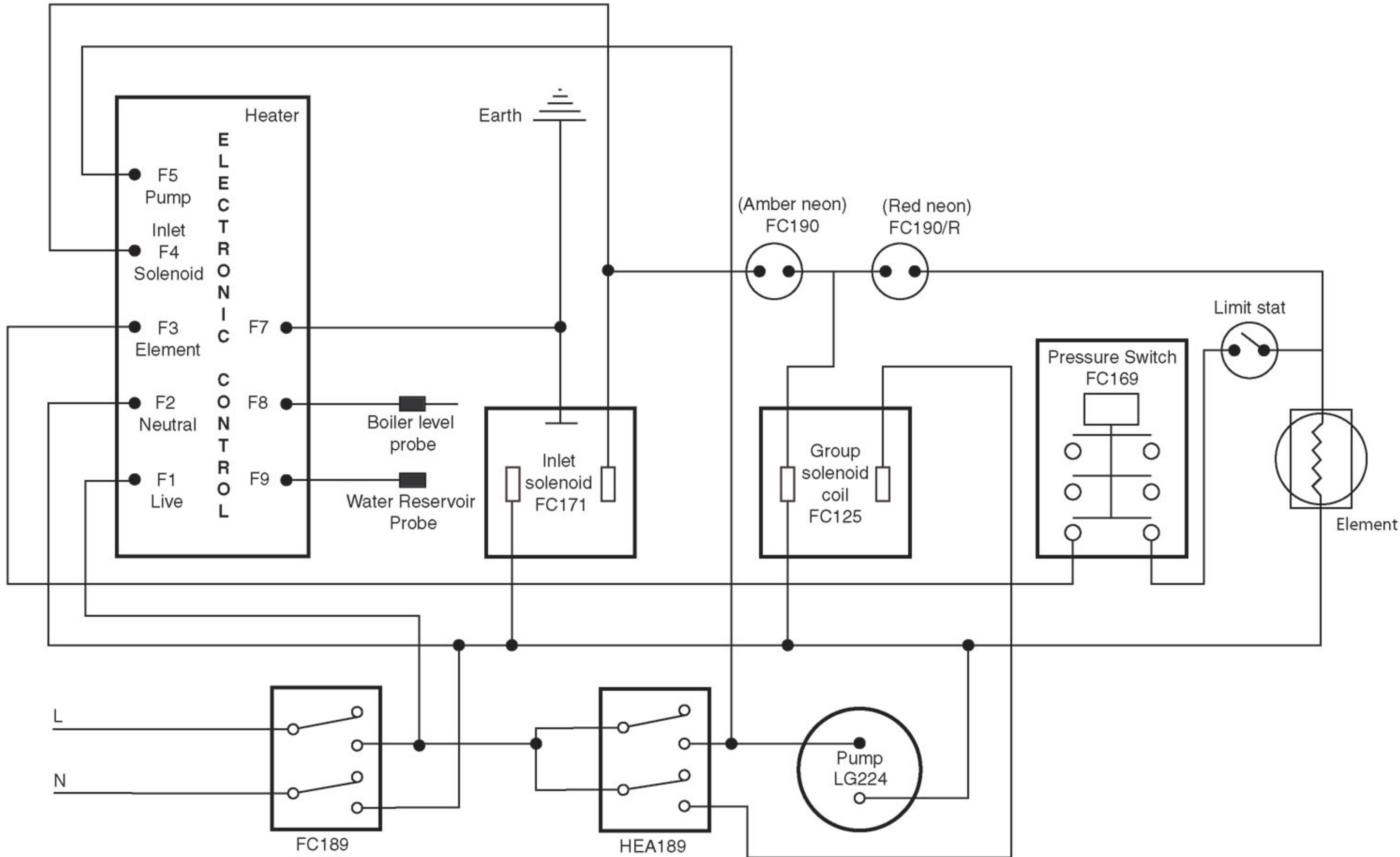
CIRCUIT DIAGRAM © Fracino 2005
