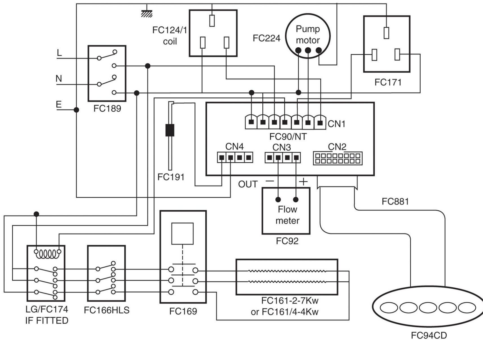
CIRCUIT DIAGRAM
