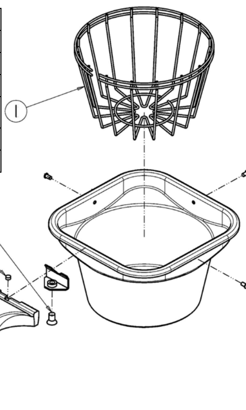
Figure 6: Brew Basket Assembly, 13" X 5", Part # B003280B1 (SQUARE)
